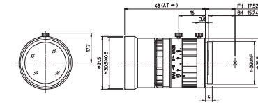
HF75HA-1B
