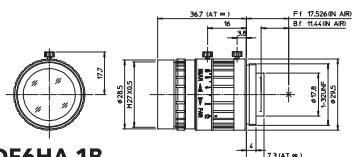
DF6HA-1B
