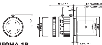
HF9HA-1B
