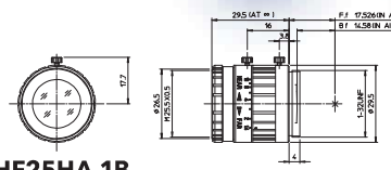
HF25HA-1B
