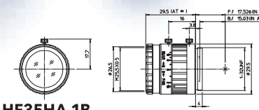
HF35HA-1B
